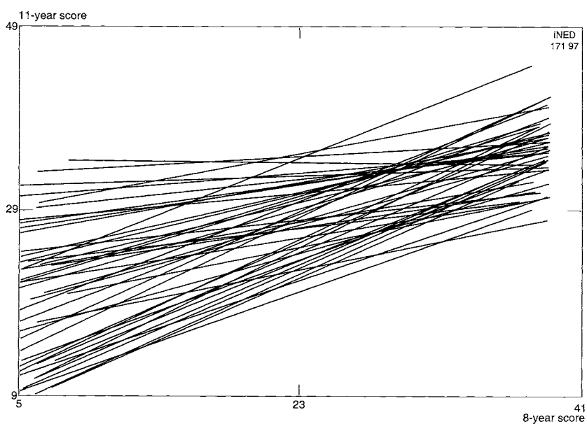
Figure 5. — Plot of predicted 11-year score by 8-year score in each school, using linear regression models applied to each school of the simulated sample (model 7)
